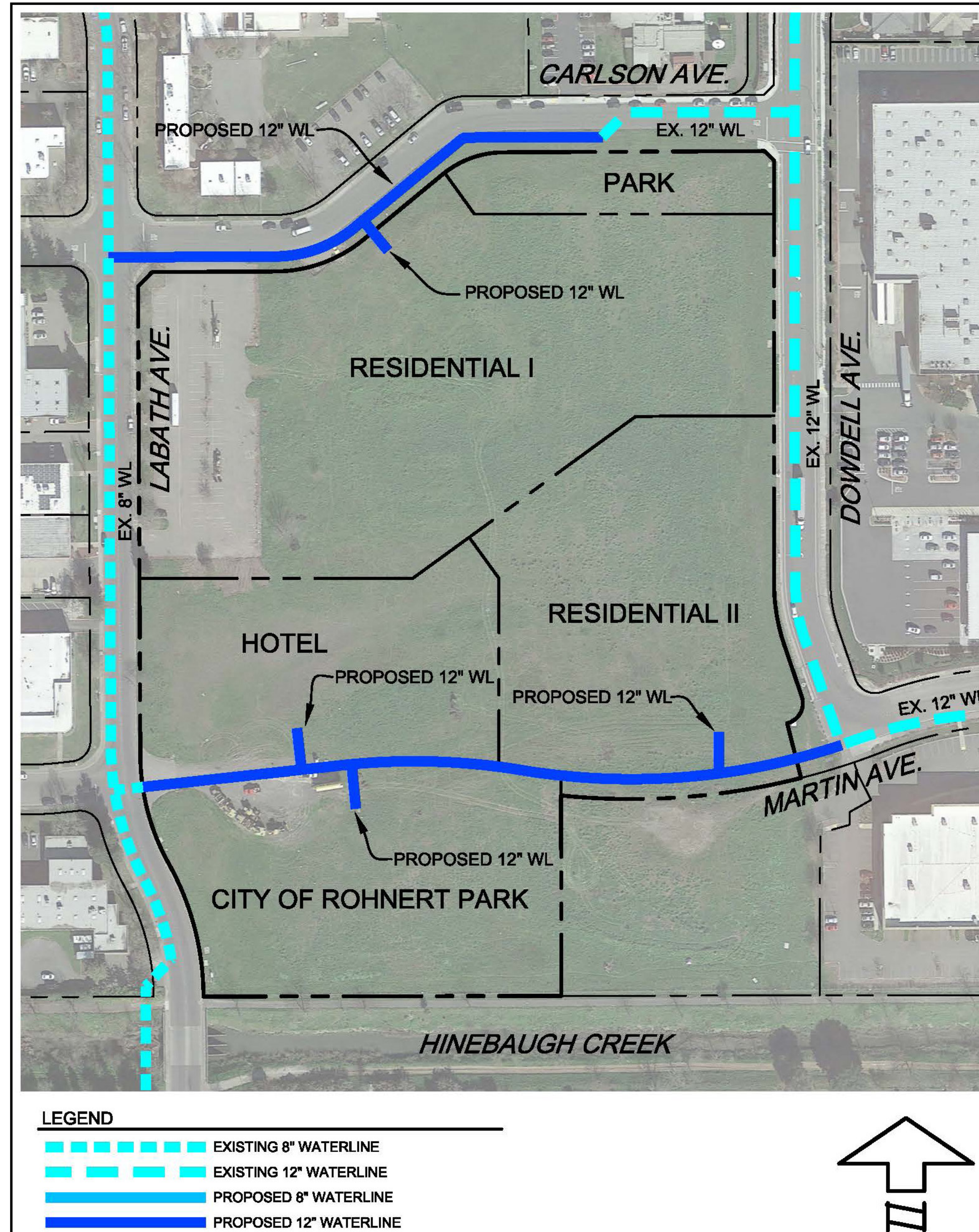
Figure 19, Water Plan
